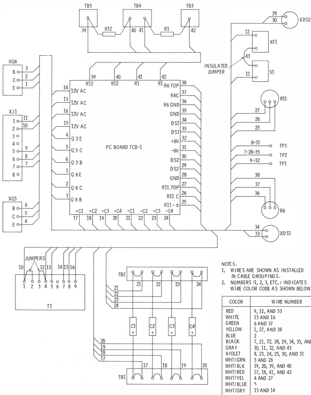
Figure 6-9. Power Supply P/O TH-83A/FGC, Wiring Diagram
